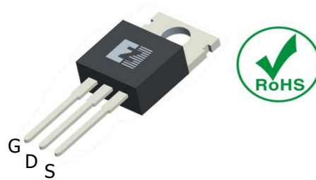
TO-220
